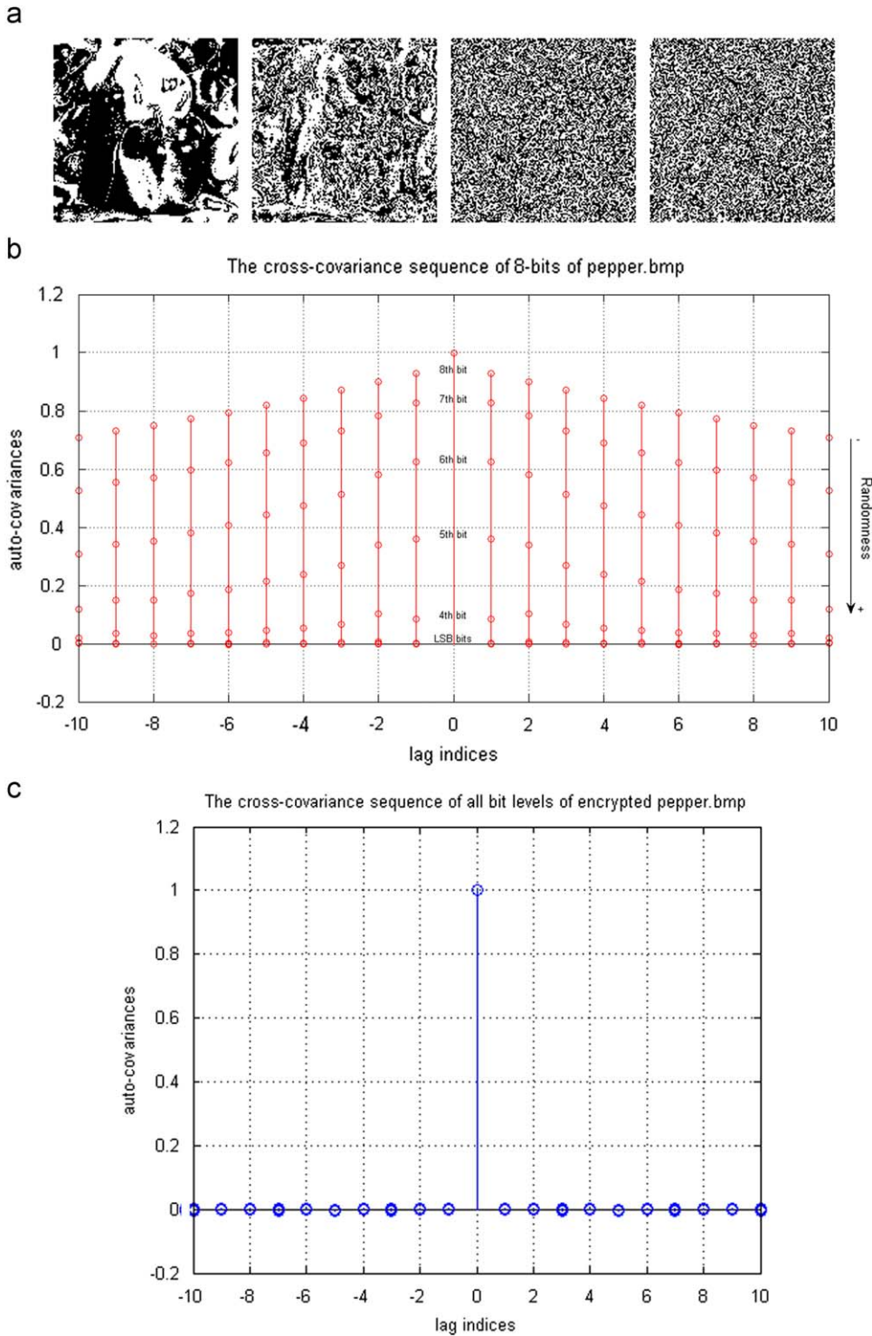
Fig. 23. Cross covariance test for randomness, (a) randomness in natural images, from left to right, original pepper.bmp 7th bit, 5th bit, 3rd bit and 2nd bit plan, respectively, (b) projection of each bit level from the plain image pepper.bmp and (c) a great randomness shown on all bit levels of the encrypted image. This phenomenon definitely helps mimic the least significant bits when embedding the encrypted secret data.
