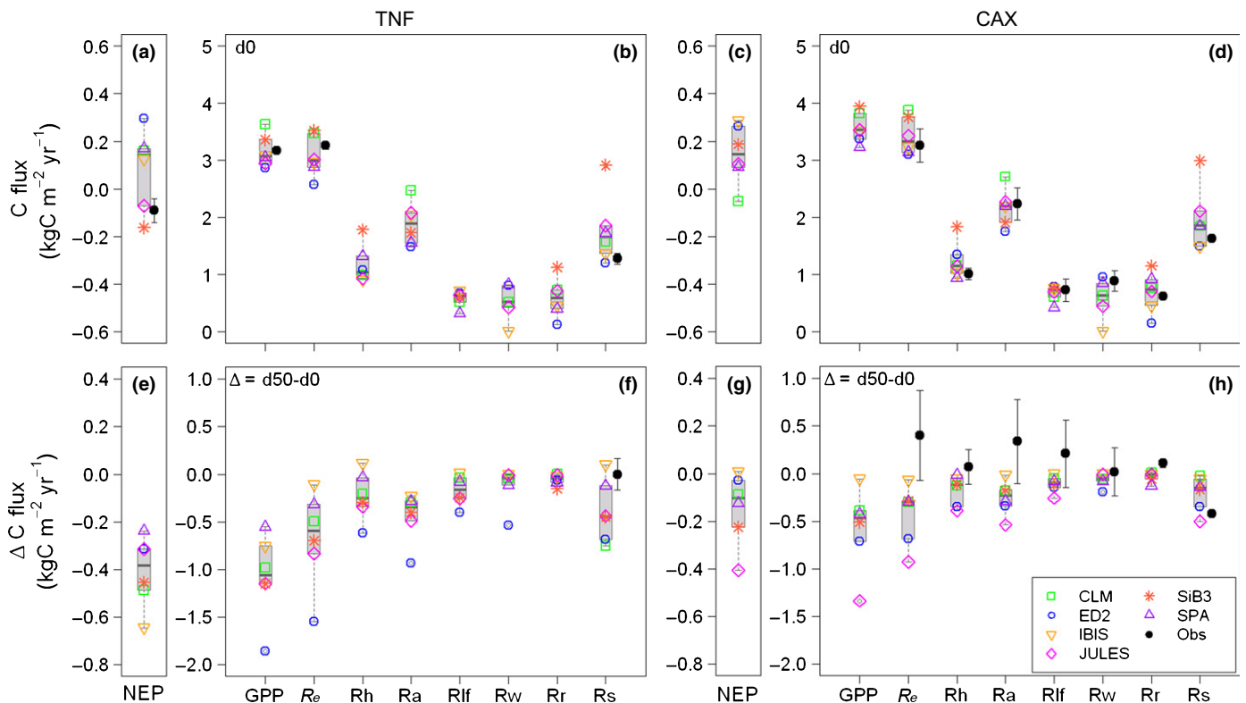
Fig. 2 Net and component ecosystem carbon fluxes ( \text{kg C m}^{-2} \text{ yr}^{-1} ) in the fourth year of the experiment for Tapajós (TNF; left side) and Caxiuaná (CAX; right side) National Forests. Carbon flux definitions and observation sources are given in Table 2. Colored symbols are model predictions and black symbols are observations (mean \pm 95% confidence interval (CI)). The control plot (d0) carbon fluxes are shown in panels (a) to (d) and the drought treatment plot (d50) fluxes are shown in panels (e) to (h). The \Delta indicates the amount the control (d0) fluxes were altered by the 50% drought treatment.
