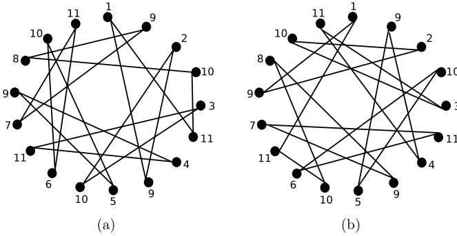
Figure 6: A 11-labeled-packing of three copies of C_{17} : (a) \sigma^1(C_{17}) , (b) \sigma^2(C_{17}) .
