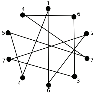
Figure 9: A 7-labeled-embedding of C_{10}
