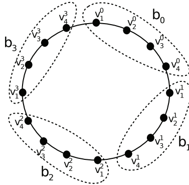
Figure 4: Partition of V(C_{16}) for k = 3 .
