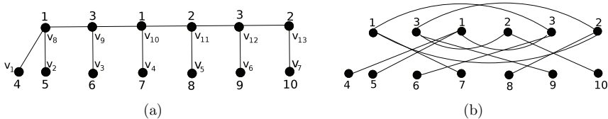
Figure 2: (a) A caterpillar T , (b) A 10-labeled embedding of T
