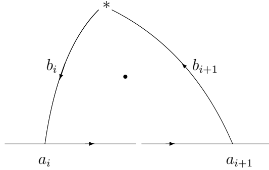
Figure 4.12: The loop \gamma_i
