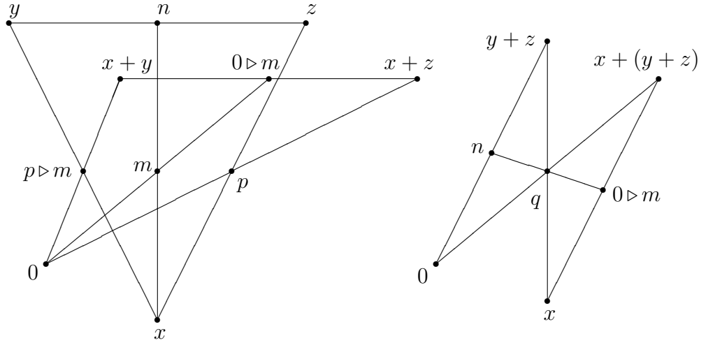
Figure 3.5: Midpoints
