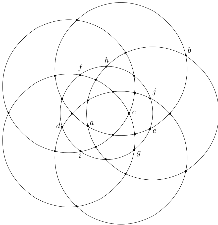
Figure 4.16: Q_2(10_{124})
