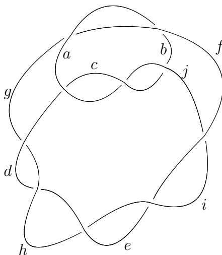
Figure 4.15: The knot 10_{124}
