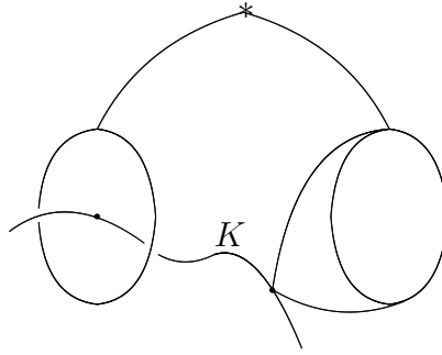
Figure 4.5: Noose boundary loops
