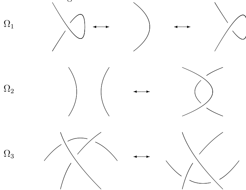
Figure 4.8: Basic knot deformations
