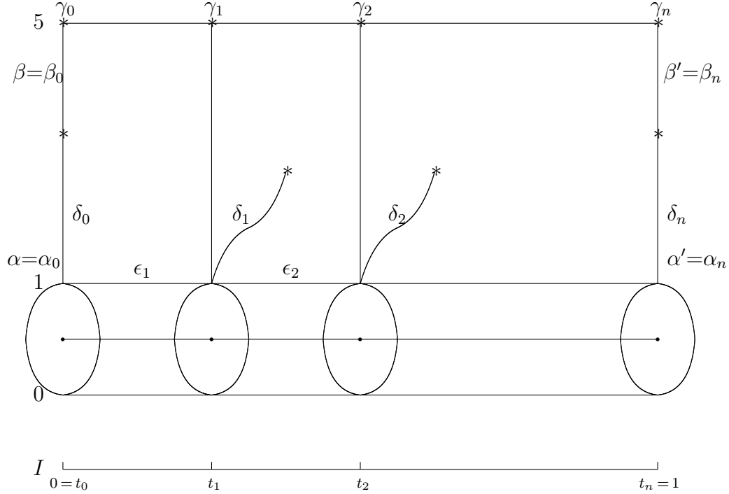
Figure 4.4: Seifert-Van Kampen noose homotopy
