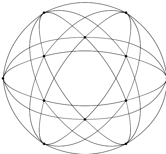
Figure 3.2: Geodesics
