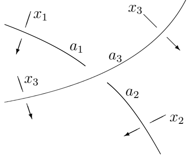
Figure 4.7: A knot crossing
