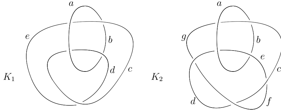
Figure 4.17: Two links with homeomorphic complements but different quandles
