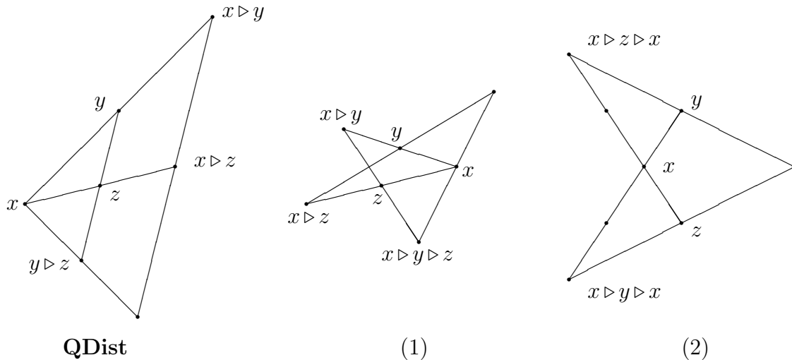
Figure 3.4: Distributivity
