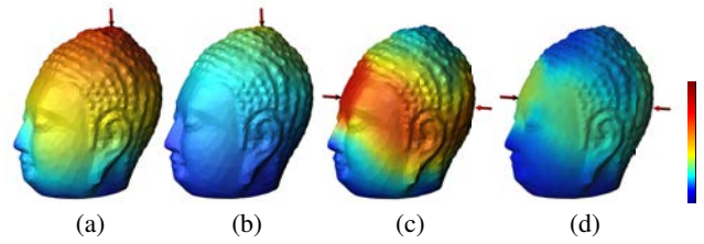
Figure 11: Deformation maps on the Buddha-Head models by the naive hollowing method (a,c) and our algorithm (b,d) under an external load of 20N. The models produced by the naive hollowing method (thickness of 1.30 mm) and ours have the same material volume ( 12.940e4 \text{ mm}^3 ), and are shown with a color visualization of the deflection displacements of their vertices.
