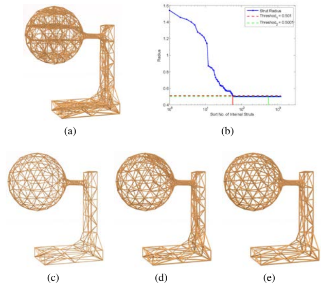
Figure 12: The effect of applying the greedy topology-cleaning to (a) the initial frame of Hanging-Ball model. Two very close thresholds 0.501mm and 0.5001mm for greedy topology-cleaning (b) lead to very different results. The first threshold (c) retains 56 internal struts such that the model has no feasible solution in the geometry optimization while the second threshold (d) retains 552 internal struts to reach a solution with the frame volume of 3.389e4 \text{ mm}^3 . In contrast, the final frame produced by our algorithm (e) has a volume of 2.875e4 \text{ mm}^3 with only 52 internal struts.
