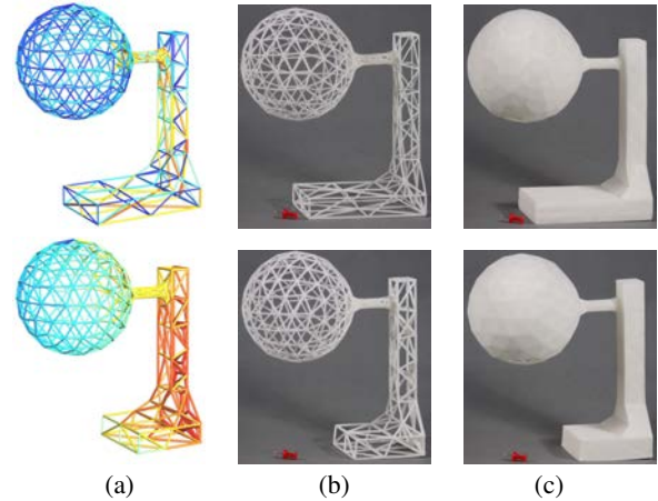
Figure 7: The Hanging-Ball model in the lower row has a smaller base than the one in the upper row. The struts in (a) are coded with the same color bar in Figure 4. For the model with a smaller base, our algorithm produces thicker struts on the vertical pillar in the right part than the counterparts in the upper row due to the balancing constraint (8). Photos of the printed naked frame and the printed objects using P-1 are shown in (b) and (c), respectively.
