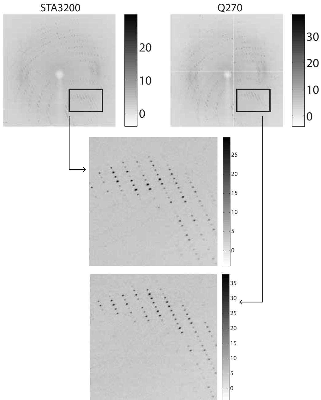
Figure 5.4: Comparison of diffraction pattern from sample Thau13. For this sample, the beam size was 100 \mu\text{m} and the sample-to-detector distances were set to give equal solid angle per pixel per detector. The boxed regions in the large images at top are magnified at bottom. The grayscale is cast in units of number of photons, with the maximum of the scale set to 5% of the maximum intensity in the frame.
