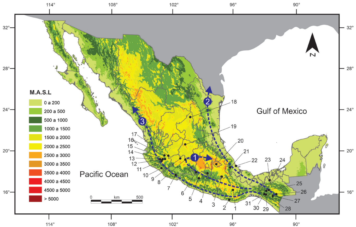
Figure 4 Localities with Eremotherium laurillardii in Mexico. For references of the localities see table 2. The arrows show the biological corridors sensu Ceballos et al. (2010): temperate corridor Transvolcanic Belt - Sierra Madre del Sur (1), and the tropical corridors Tamaulipas - Central America Gulf Lowlands (2), and Sonora - Central America Pacific lowlands (3).
