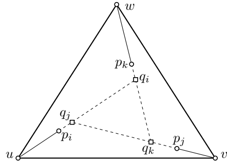
Figure 4: Always O(n^3) pseudo-triangles, second case.
