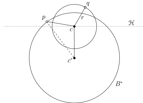
Figure 3: Proof of Theorem 4.
