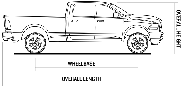
RAM CREW CAB WITH 8' BOX SHOWN
