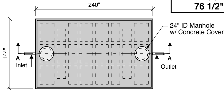
Top View
