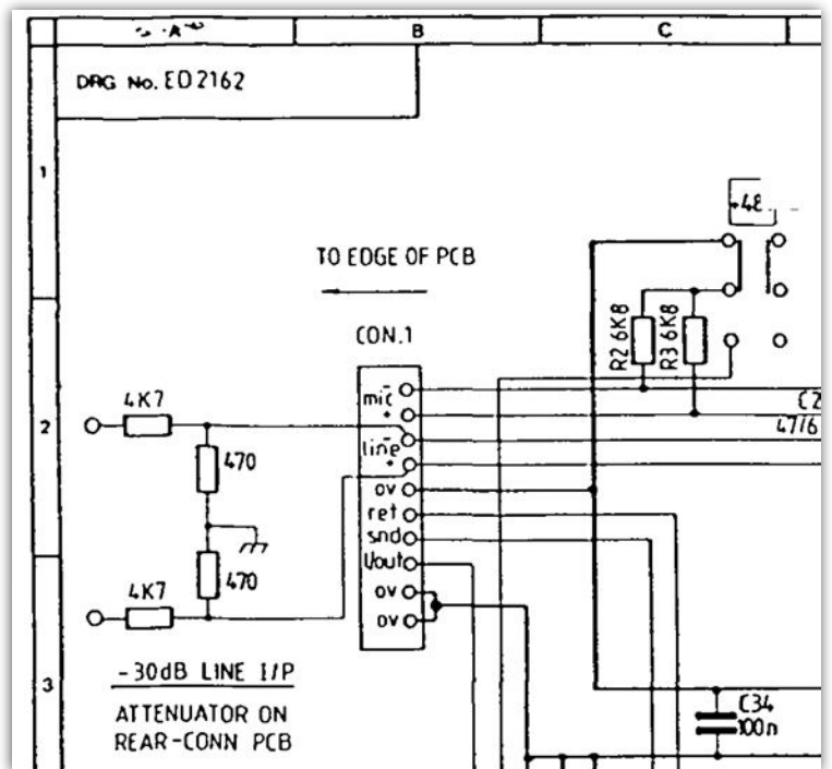
The Soundcraft 600's padding of line-level sources so they can be run through the mic amps, as indicated in this excerpt from the manual's block diagram, is a common and pragmatic arrangement — and really not as big a 'problem' as some purists may suggest!
