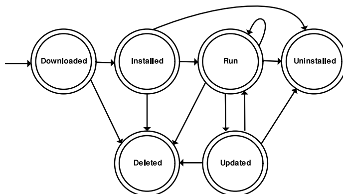
Figure 1. Program lifecycle.
