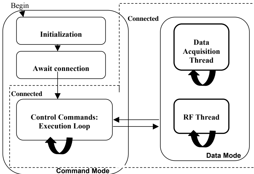
Fig. 5. Software Architecture of the Device (State Machine)
