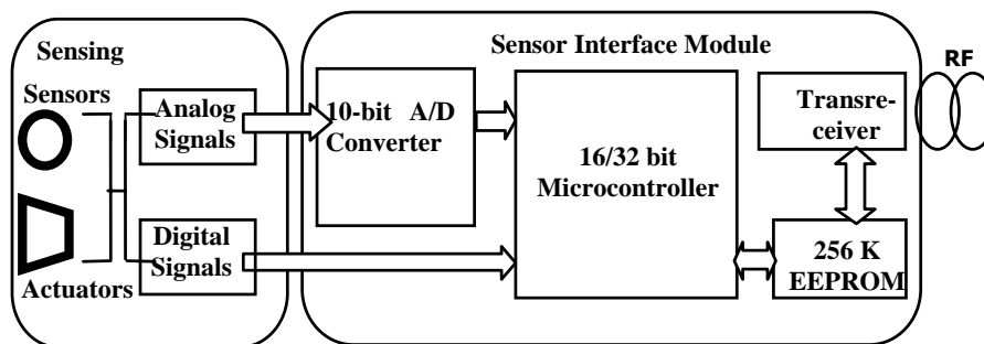
Fig. 4. Hardware design of Intelligent Sensor
