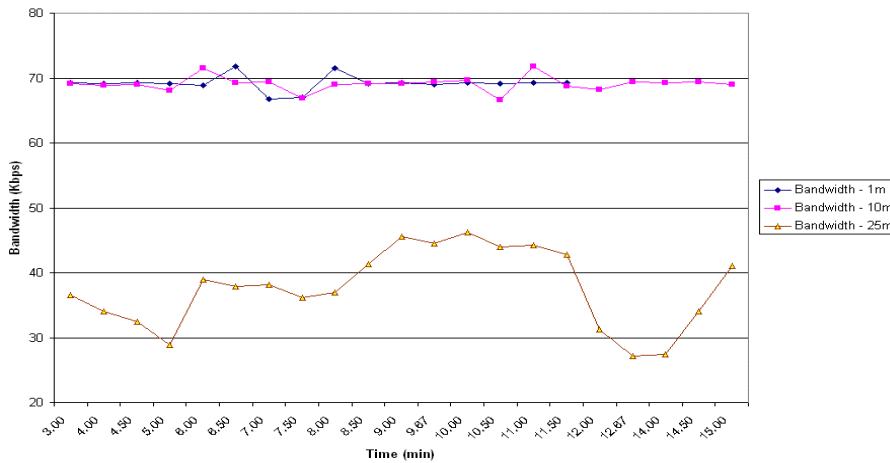
Fig. 11. Bandwidth Performance with distance
