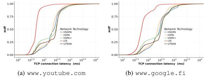
Fig. 7: TCP connect time towards www.youtube.com and www.google.fi by radio technology. The distribution exhibits similar pattern for www.elisa.net and www.facebook.com , too.
