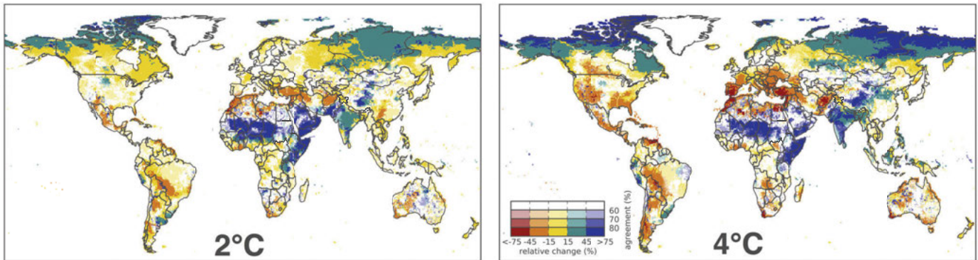
Figure 2.7: Relative change in annual water discharge for a 2°C world and a 4°C world.
