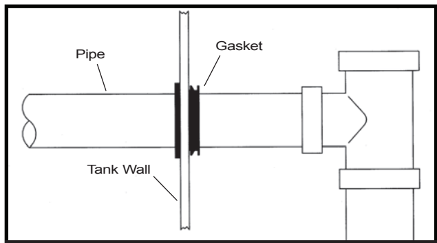
FIG.2 Gasket Detail
