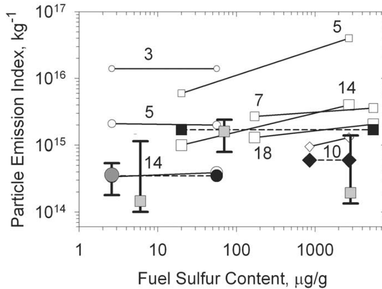
Figure 8. Emission index of detectable particle numbers in dissipating contrails for various aircraft and lower detection limits d of particle diameters versus FSC, behind the ATTAS (squares), B737 (circles), and A310 (diamonds). The open symbols with solid lines indicate data for volatile particles of various sizes in nanometers, as indicated; the symbol sizes are proportional to the particle diameters. The solid symbols with dashed lines approximate the mean soot particle emission indices measured for the three aircraft in noncontrail plumes. The gray symbols with error bars denote the number of ice particles formed per kilogram of fuel burned in contrails for the B737 (S6) and the ATTAS (S4 and S6). Data for B737 from S6 at 3, 5, and 14 nm and ice particles for 2.6 \mu\text{g/g} FSC at 0.4 s plume age; ATTAS (S2) 7 and 18 nm, 20 s; ATTAS (S4) ice particles for 6 and 2830 \mu\text{g/g} FSC, 10 s; ATTAS (S5) 5 and 14 nm, 20 s; ATTAS (S6) ice particles assigned to a mid FSC of 70 \mu\text{g/g} , 1 and 20 s; A310 (S4) 10 nm, 5 s.
