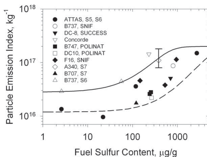
Figure 7. Particle number emission index (PEI) of detectable volatile particles in noncontrail plumes versus FSC from various measurements, normalized to plume age 3 s, CPC cutoff 5 nm, and various sulfur conversion fractions \epsilon and emission indices of condensable organic matter, EI_{OM} , see Table 10, adjusted to approximate the measured concentrations as closely as possible. The result for the Concorde represents the value computed from the lower bound of the reported range of nonvolatile particle EIs [Fahey et al. , 1995]. The symbol and the error bar for the A340 represent the best estimate and the range derived from the particle concentrations measured. The curves emphasizing the trend of observed PEI with increasing FSC are model results at the same values of plume age, cutoff, and EI of CIs of 2 \times 10^{17} \text{ kg}^{-1} , and different EI_{OM} and \epsilon values: 20 \mu\text{g/g} and 0.5% for dashed curve, and 30 \mu\text{g/g} and 8% for solid curve. From Kärcher et al. [2000] with additional data for the B737, A340, and B707 (S6 and S7).
