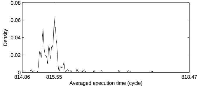
Fig. 3. Distribution of execution times for an unprotected openSSL implementation of AES. The execution times are averaged, regarding the value of one fixed byte of the plaintext, over a large number of random plaintexts (measurements have been taken according to [Ber]). In this example, two visible peaks suggest higher density around two timing accesses.
