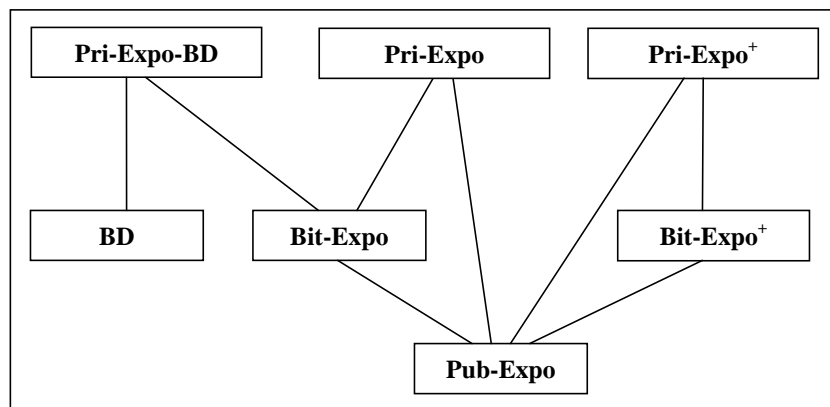
Figure 6: Hierarchy of The Protocols for Exponentiation
