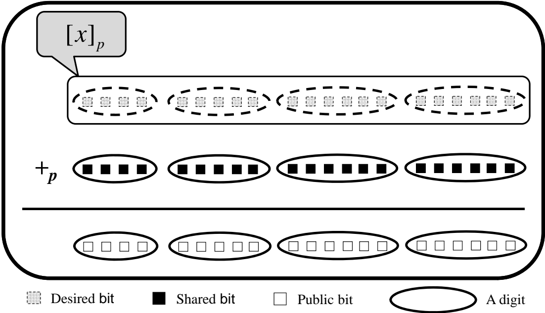
Figure 9: Intuition behind Hybrid-base Digit-Decomposition and Digit-Bit-Decomposition
