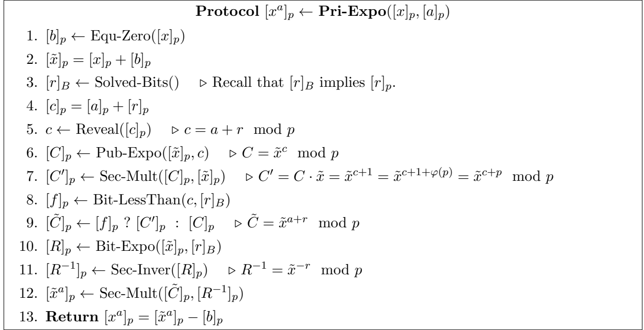
Figure 4: The Private Exponentiation Protocol without BD
