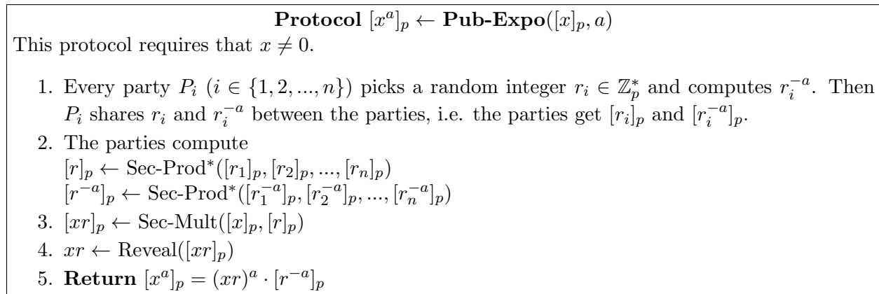
Figure 1: The Public Exponentiation Protocol
