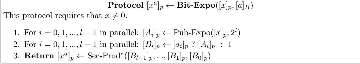
Figure 2: The Bit Exponentiation Protocol
