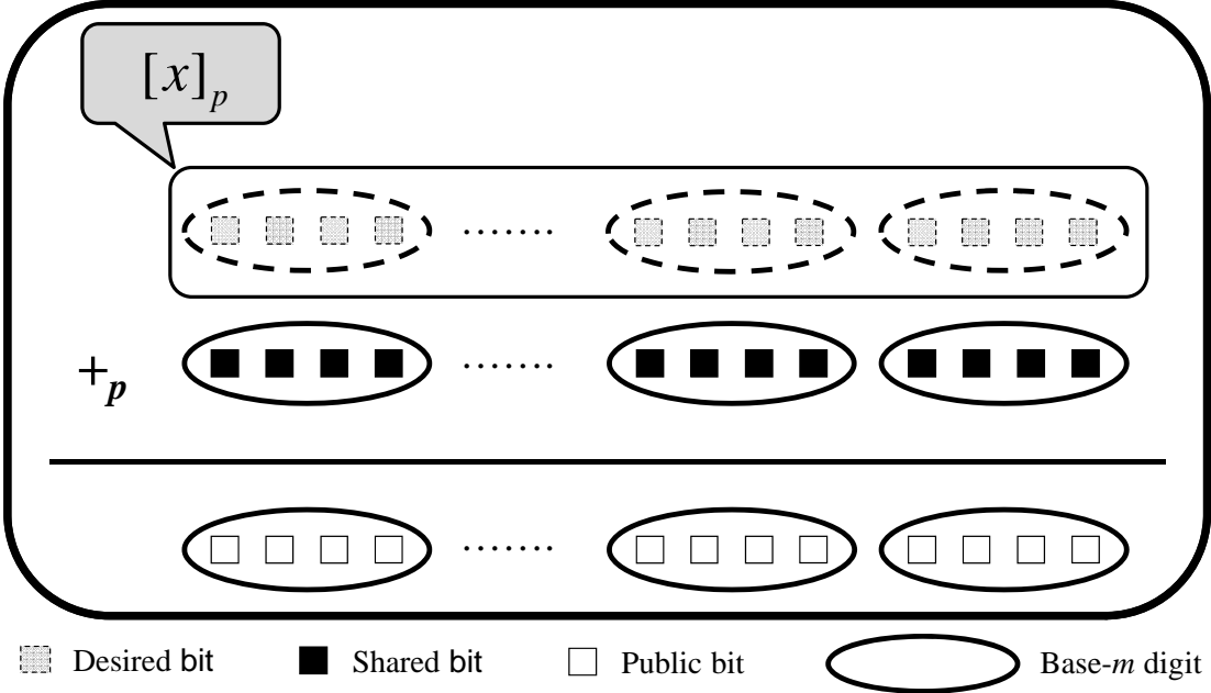
Figure 8: Intuition behind Base- m Digit-Decomposition and Digit-Bit-Decomposition
