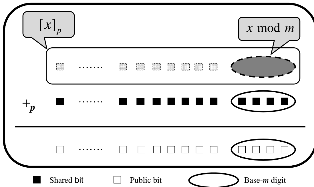
Figure 11: Intuition behind our Pub-MR + (·) Protocol
