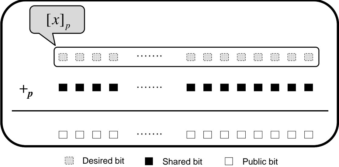
Figure 7: Intuition behind BD
