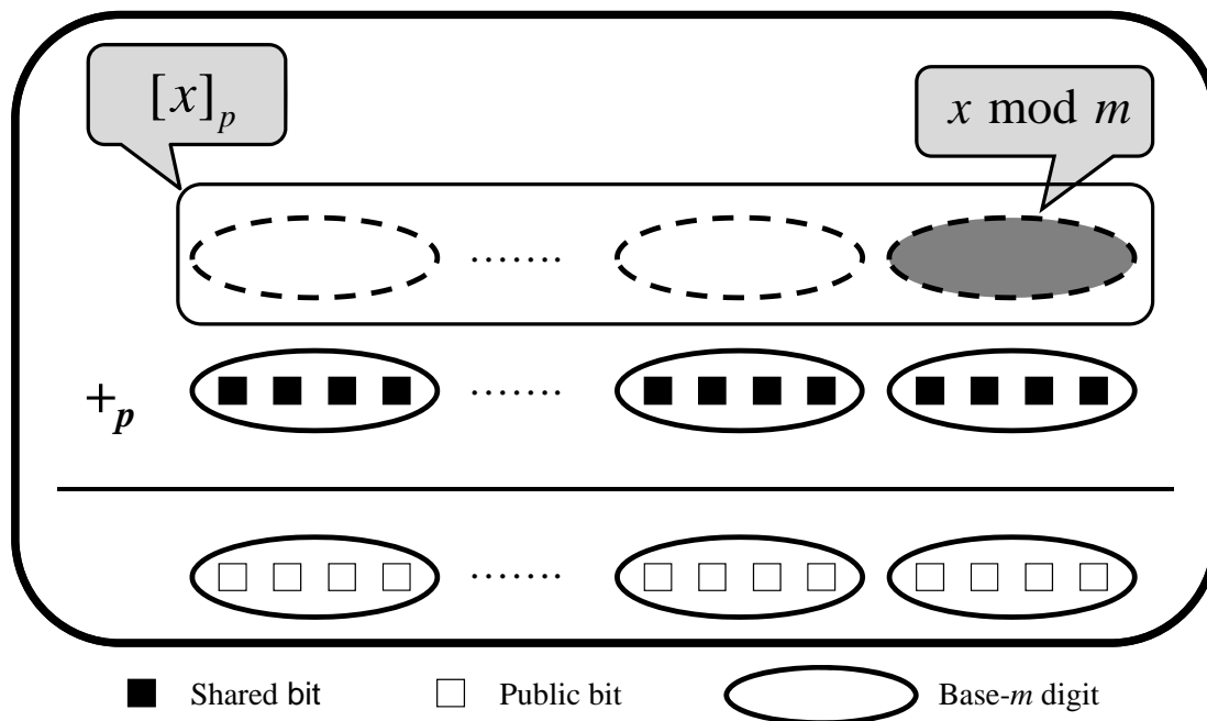
Figure 10: Intuition behind the Pub-MR( \cdot ) Protocol in [NX10]
