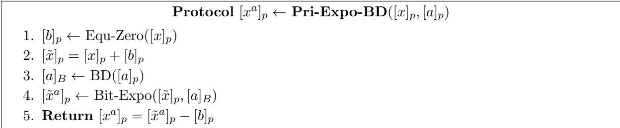
Figure 3: The Private Exponentiation Protocol with BD
