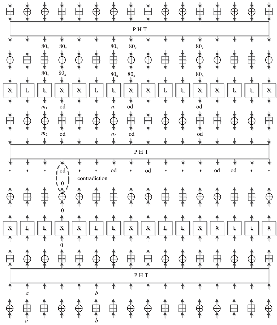
Fig. 1. 2.75-Round Impossible Differential of SAFER+
