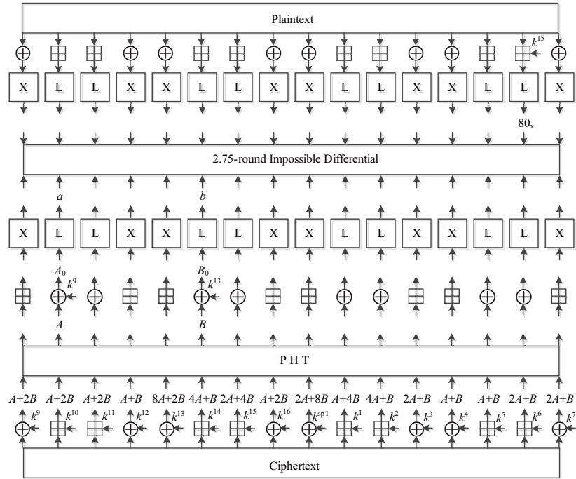
Fig. 3. Impossible Differential Attack on 4-Round SAFER+/128
