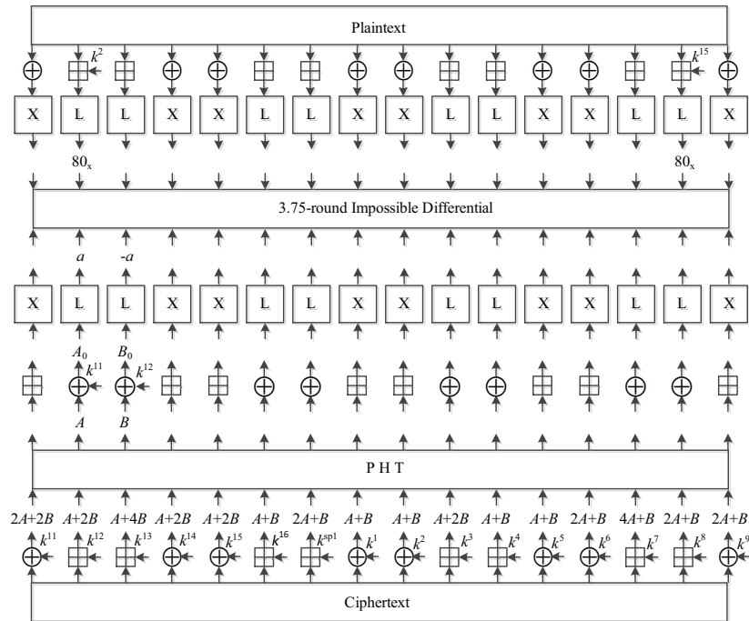
Fig. 5. Impossible Differential Attack on 5-Round SAFER++/128
