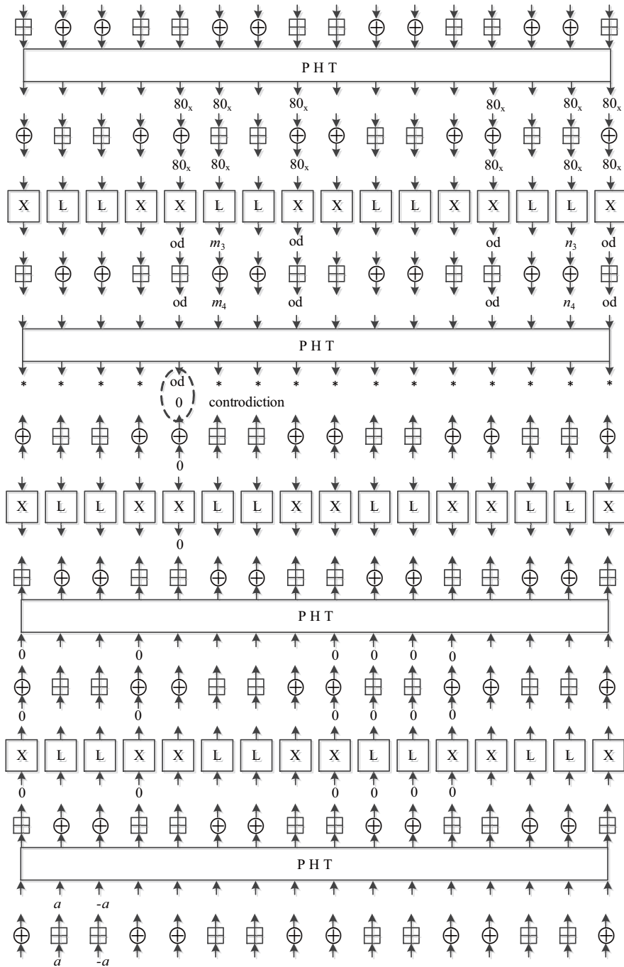
Fig. 2. 3.75-Round Impossible Differential of SAFER++
