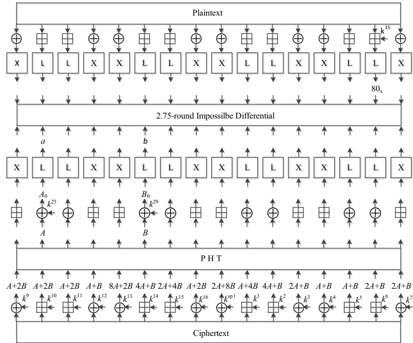
Fig. 4. Impossible Differential Attack on 4-Round SAFER+/256
