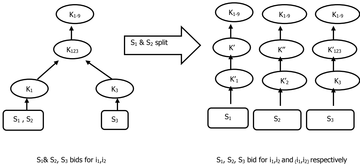
Fig. 4 : Key management for split
