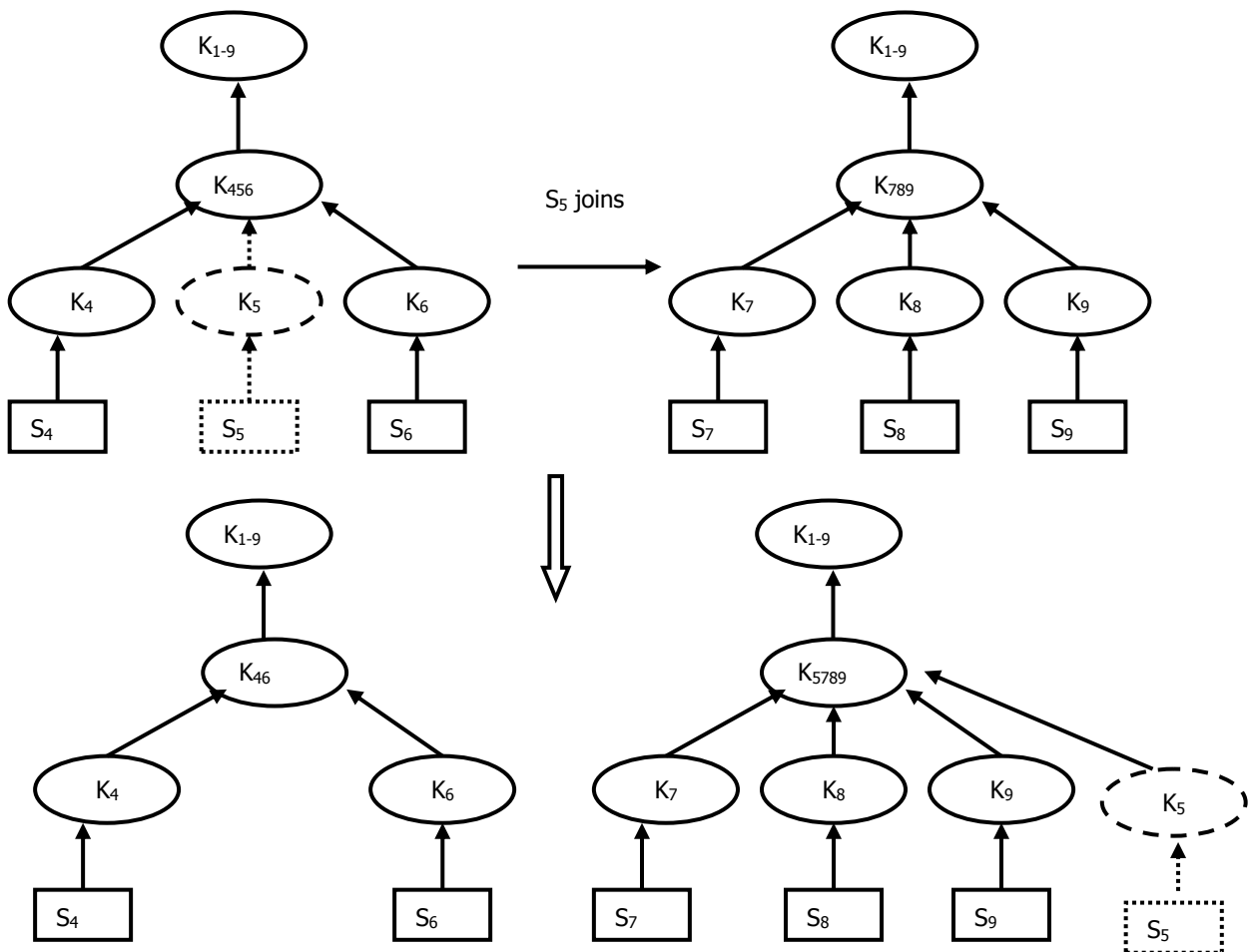
Fig. 2 : Key management for change of subgroup
