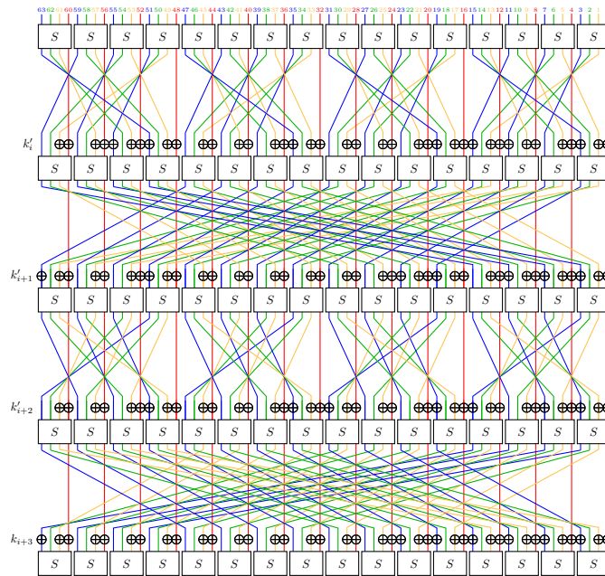
Figure 11: Fixsliced representation of GIFT-64 over 4 rounds. Each color refers to a slice.
