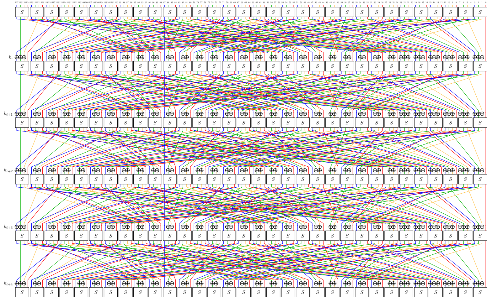
Figure 12: Classical representation of GIFT-128 over 5 rounds. Each color refers to a slice.
