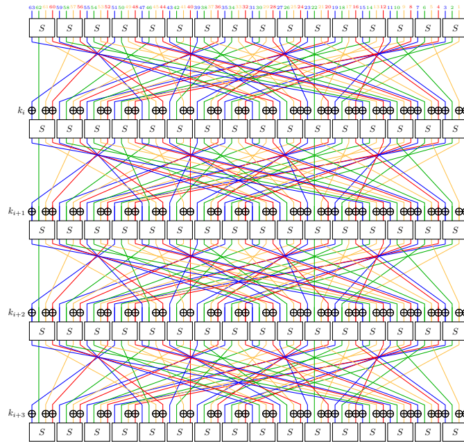
Figure 10: Classical representation of GIFT-64 over 4 rounds. Each color refers to a slice.
