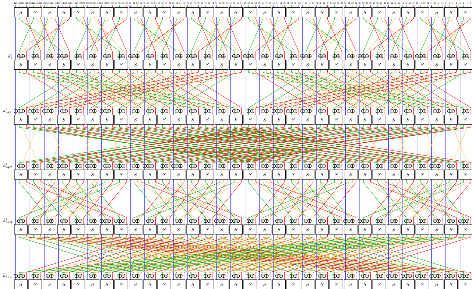
Figure 13: Fixsliced representation of GIFT-128 over 5 rounds. Each color refers to a slice.
