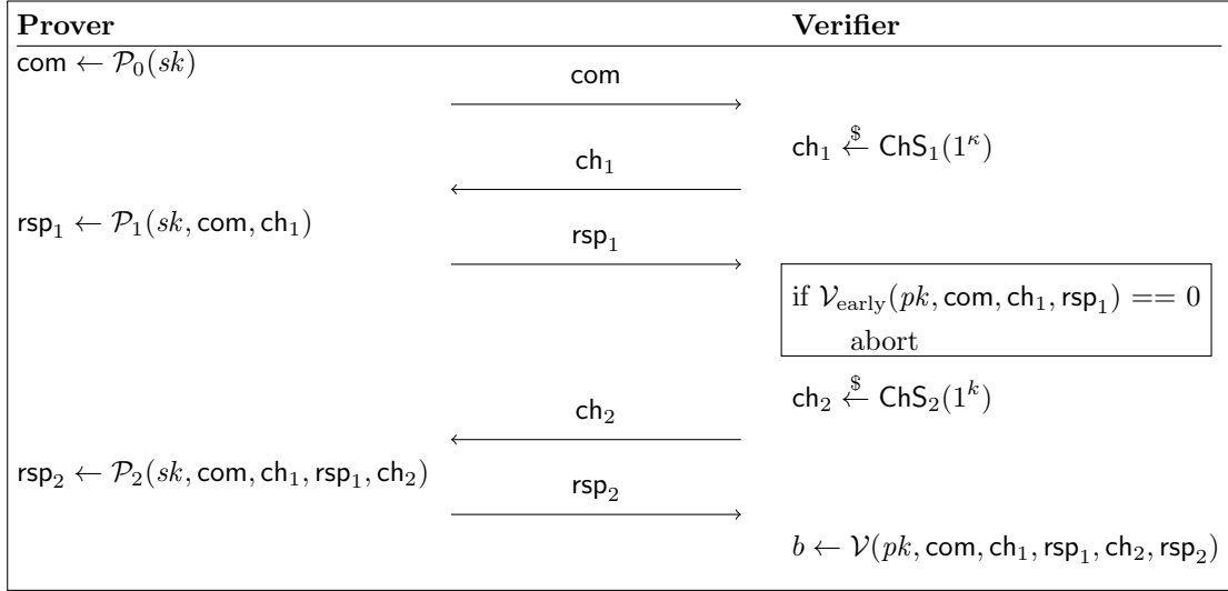
Figure 2: A 5-pass identification scheme with capability for early abort.
