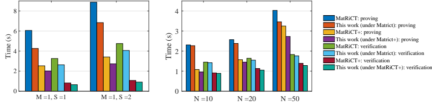
Fig. 3: Time cost of balance proofs. Fig. 4: Time cost of ring signatures.
