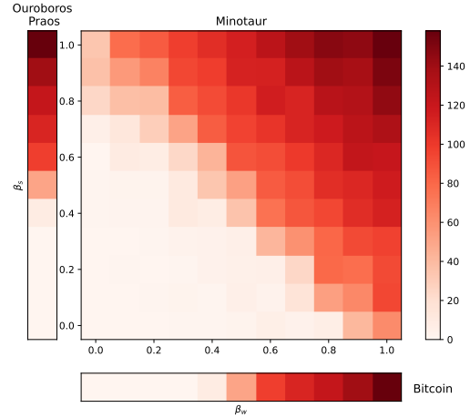
Figure 6: Longest private chain in private attacks with various adversarial stake fraction \beta_s and adversarial mining power fraction \beta_w on Minotaur, Ouroboros Praos, and Bitcoin. When \beta_s + \beta_w < 1 and either \beta_s or \beta_w is close to 1, the private chain in Minotaur is way shorter, meaning that it remains secure whereas Ouroboros Praos and Bitcoin are insecure.
