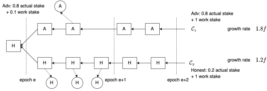
Figure 10: A long range attack on the longest chain rule.
