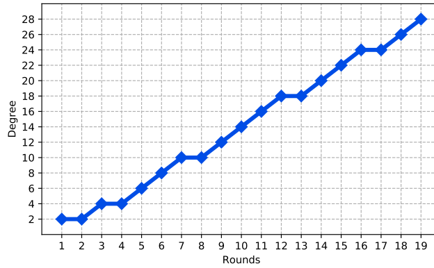
Figure 3: Algebraic degree of MIMC 3 .
