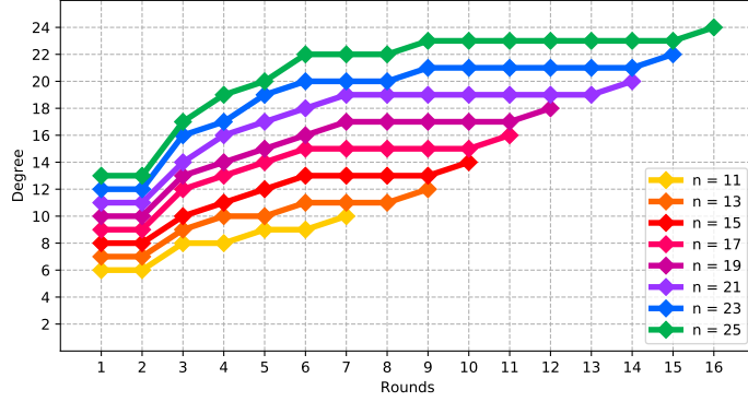
Figure 8: Algebraic degree of \text{MIMC}_3^{-1}
