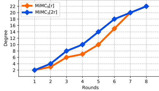
Figure 7: Comparison of algebraic degree for rounds r of \text{MIMC}_9 and for rounds 2r of \text{MIMC}_3 ( n = 23 ).
