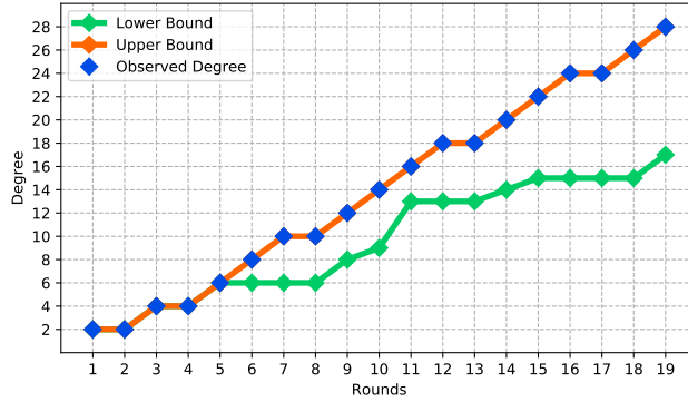
Figure 4: Comparison between the observed degree and the bounds (for n \geq 31 ).
