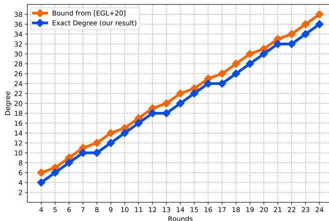
Figure 6: Comparison of the exact value of B_3^r given in Corollary 4.11 with previous work.
