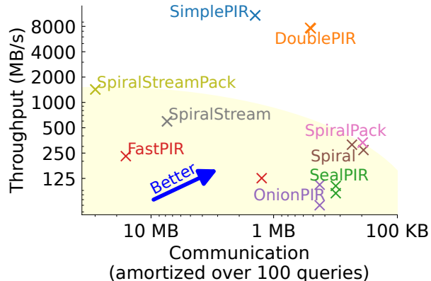
Figure 6: Throughput vs. per-query communication, on a 1 GB database. For each PIR scheme, we display the communication and the corresponding throughput for two choices of entry size: one that maximizes throughput, and another that minimizes communication. (For schemes displayed only once, both entry sizes are the same.) The communication cost is the total (i.e., offline and online) communication, amortized over 100 queries. We highlight prior work in yellow.
