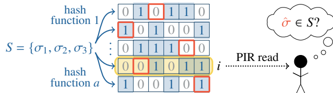
Figure 4: Our data structure for private, approximate set membership with adversarial soundness, when instantiated with a set S consisting of three strings and with a = 5 hash functions. We highlight in blue the bits of the data structure that are set, in red the bits that the query string \hat{\sigma} maps to, and in yellow the area covered by the client’s PIR read, when the client probes the i -th one-hash-function Bloom filter.
