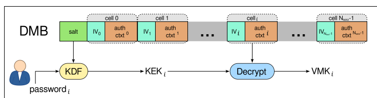
Fig. 5: (Legacy) Shufflecake’s Device Master Block (DMB).
