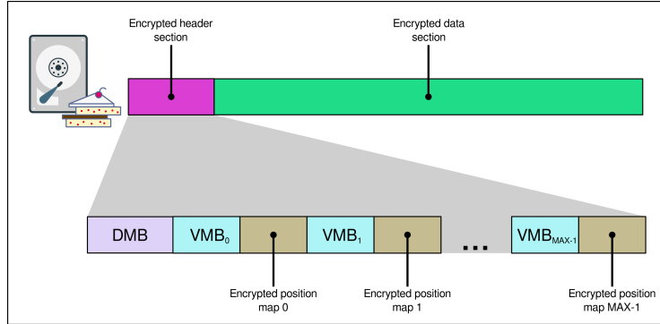
Fig. 3: (Legacy) Shufflecake’s disk layout overview.
