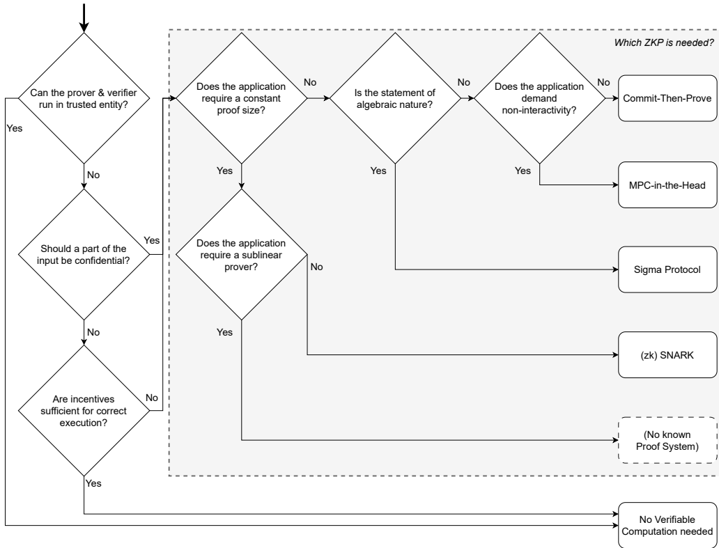
Fig. 1: A flow chart to determine which proof system is the appropriate technical solution to establishing cryptographic verifiability of outsourced computations. We assume that the computation is executed between a prover and a verifier .
