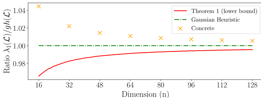
Fig. 3. The asymptotic existence bound of Theorem 1 versus a concrete computation for the genus of the lattice \mathbb{Z}^k \oplus 521\mathbb{Z}^k . This genus contains a large class of random q -ary lattices [BDG23] or of NTRU lattices with q = 521 . All values are normalized by the Gaussian Heuristic.
