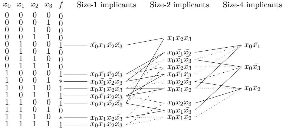
Figure 1: Generation of prime implicants with the QuineMcCluskey algorithm. Prime implicants are in bold.
