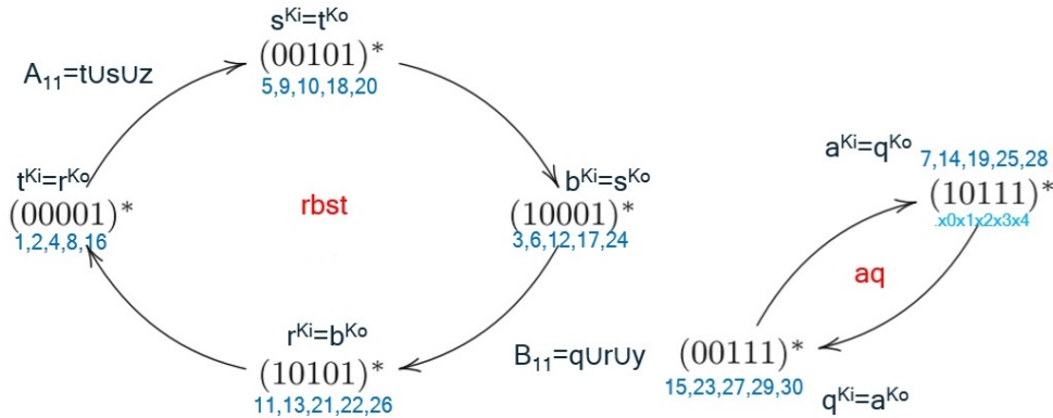
Fig. 3. State diagram for Keccak S-box excluding 2 special points, with 20 points of order 4 and 10 points of order 2, grouped into sets of 5 canonical states with all their rotations, based on Fig. 1 page 1394 in [ScDa24] and annotated with special distinguished sets defined in this paper.
