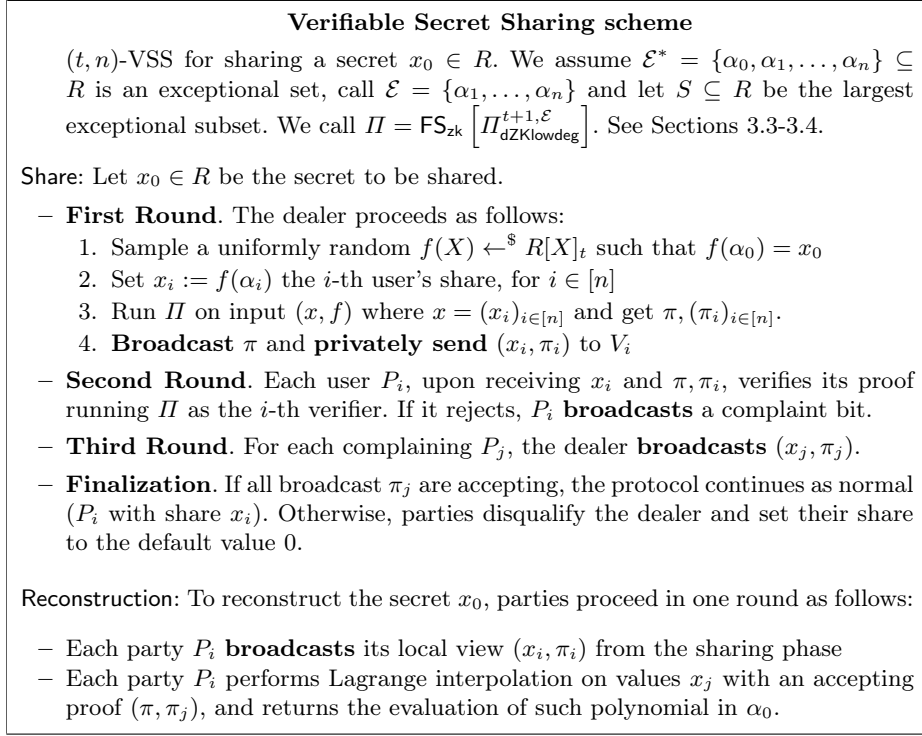
Fig. 5. Verifiable Secret Sharing from non-interactive distributed ZKP.
