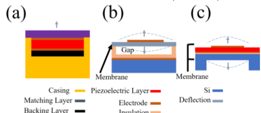
Fig. 1. Typical architectures of (a) a bulk piezoelectric transducer, (b) a capacitive micromachined ultrasonic transducer and (c) a piezoelectric micromachined ultrasonic transducer (after [8]).
