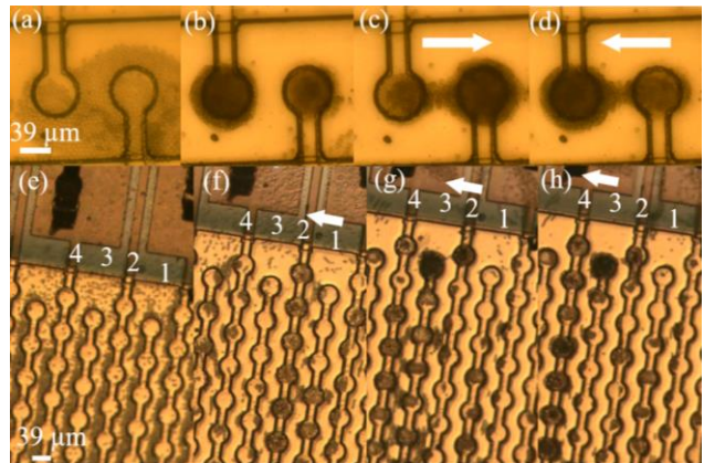
Fig. 9. Manipulation of 4 \mu\text{m} silica beads using two elements from the E1 (a)–(d) and E20 (e)–(h) PMUT designs. The images show the \text{SiO}_2 beads when (a) elements are off, (b) both elements are turned on, (c) when the left element is switched off and the right element remains on, and (d) when the right element is switched off and the left element is switched on. Beads move from the element that is turned off to the element that is turned on. This technique was used when manipulating the beads with the E20 design, where beads were trapped and moved from element 1 to element 4. The white arrows indicate the direction of particle movement. Note the scalebars are consistent between (a)–(d) and (e)–(h).
