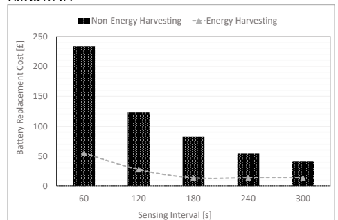
Fig. 10. Comparison of battery replacement cost when exploiting energy harvesting sources in industrial environment
