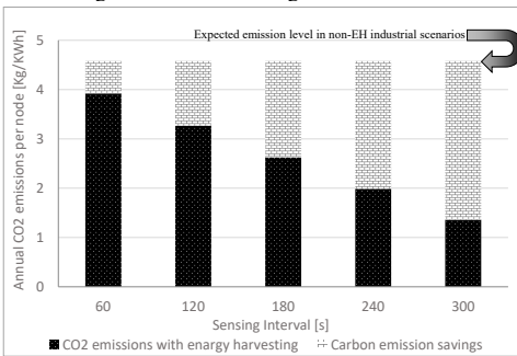
Fig. 14. Annual carbon emission savings per node against different sensing intervals
