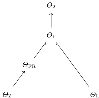
Fig. 1. Comparison of existing transformations for proving termination.
