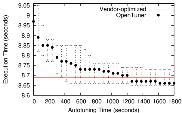
Figure 9: High Performance Linpack: Execution time (lower is better) as a function of autotuning time. Aggregated performance of 30 runs of OpenTuner, error bars indicate median, 20th, and 80th percentiles.
