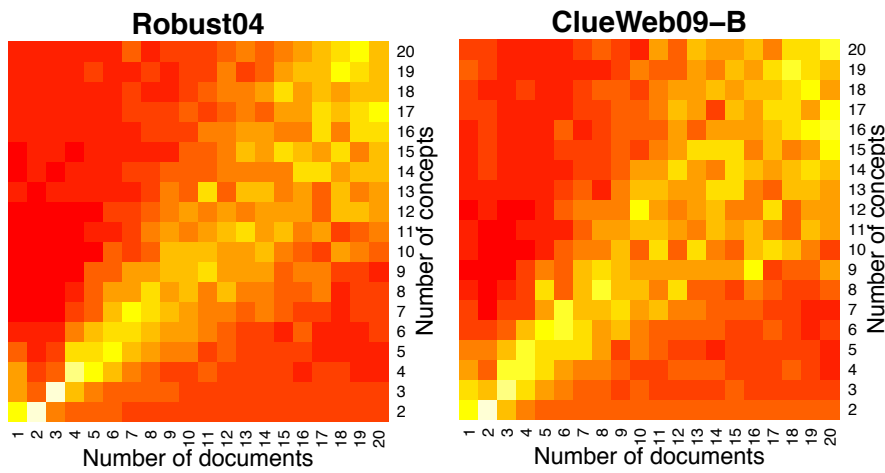
Figure 1. Number of queries for which \hat{K} where modeled, function of the number of pseudo-relevant feedback documents. A bright yellow square means a high number of queries, whereas a red square means that no query is associated to the corresponding values
