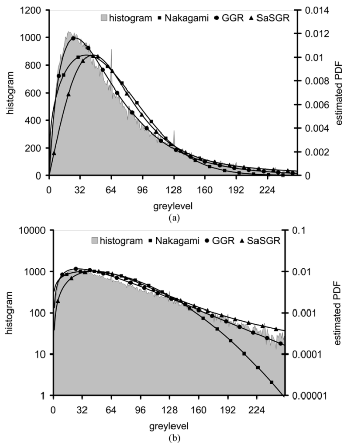
Fig. 5. Plots of the image histogram and of the estimated GGR, SaSGR, and Nakagami PDFs for the “Feltwell-CHH” data set: (a) linear scale and (b) logarithmic scale.
