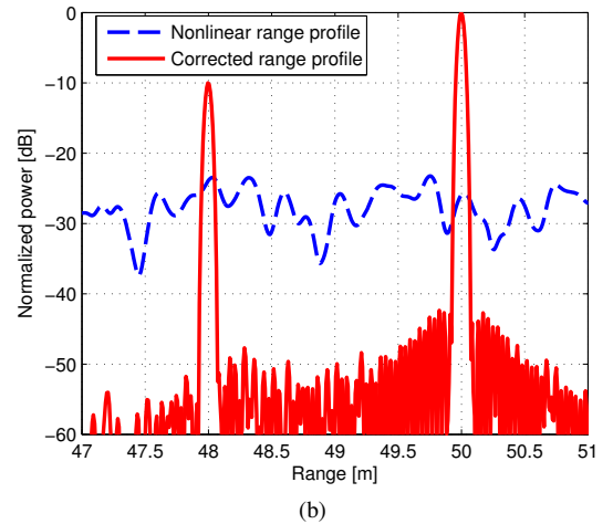
Fig. 4. Range profiles simulation results: (a) 0-100m range, (b) detailed 47-51m range. In the nonlinear profile five targets are completely indistinguishable. The corrected profile leads to a resolution near the theoretical limit and improves the signal to noise ratio.
