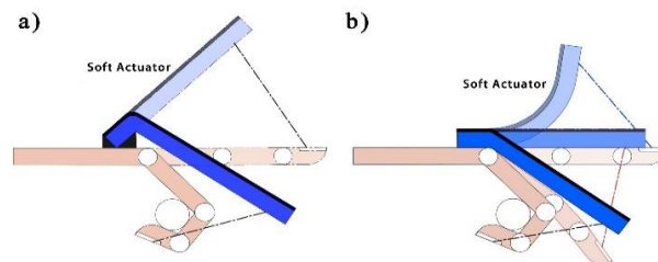
Fig. 3. Comparison before and after introducing a positive pre-bending deformation. a) The actuator has no bending deformation at the full extension state and negative bending at the full grasping state. b) The actuator has positive bending at the full extension state, no bending at the intermediate state, and negative bending at the full grasping state.
