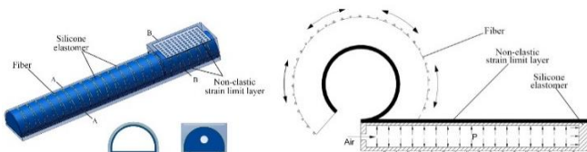
Fig. 2. Inflation of a soft actuator with strain limiting layer and radial reinforcement. a) 3D illustration. b) Bending with inflated air.
