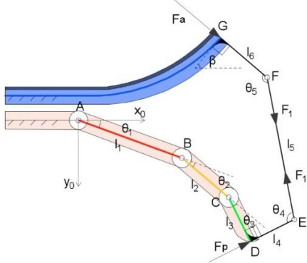
Fig. 5. Schematic diagram for constructing the kinematic model
