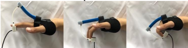
Fig. 14. Measuring fingertip forces during repeated grasping motion
