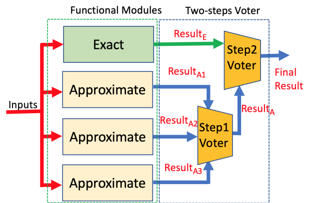
Figure 1: The Proposed Quadruple Modular Redundancy (QMR) and Two-Steps Voter
