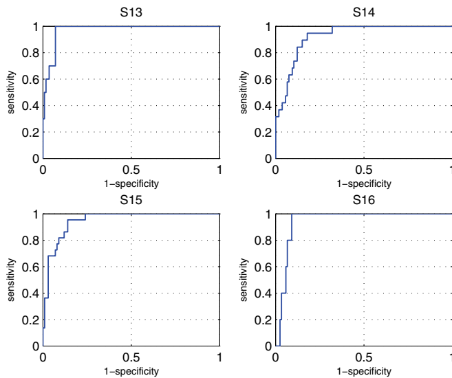
Figure 7: Test ROC curves for segments 13 through 16: BNT.
