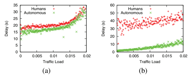
Figure 6: Average delay for humans and autonomous vehicles as a function of traffic level for FCFS-LIGHT with 5% human, SINGLE-LANE(a) and 50% human, ALL-LANES(b).
