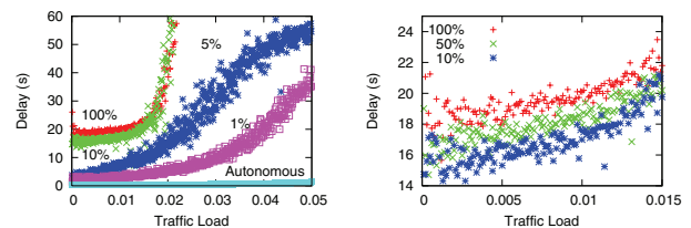
(a) Delays decrease with decreasing proportions of human drivers. (b) A closeup of the ALL-LANES results.
