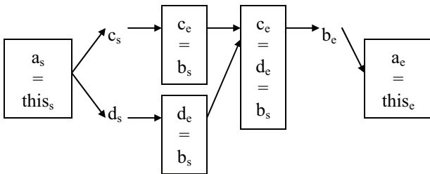
Figure 1: The directed graph representation for 'Camel-Sit_Spin'. Edges (a_s, a_c) , (a_s, b_s) , (c_c, a_c) , and (d_c, a_c) are omitted in the graph.
