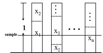
Figure 1: Comb Sampling
