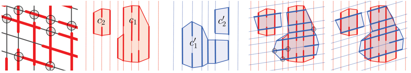
(a) An overlay of two sensor measurements with mismatches that are indicated by circles. (b) A partition of the measurement from Figure 1c, which consist of two clusters c_1 and c_2 . (c) A partition of the measurement from Figure 1d, which consist of two clusters c'_1 and c'_2 . (d) Initial match based on the spatial structures of the clusters. There are 4 mismatches. (e) Result after fine-tuning with a local search.
