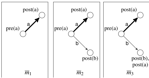
Figure 1: Example 1-bounded models, where bold lines indicate actual paths.
