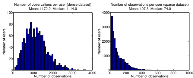
Figure 1: Number of observations per user. The left plot represents a dense mobile carrier dataset and the right plot represents a sparse mobile ad exchange dataset. The dense dataset has 15 times more observations per user than the sparse dataset.
