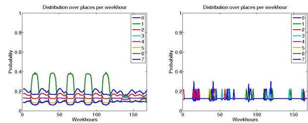
Figure 7: Posterior and empirical place distributions for the sparse dataset. The left plot is the place distribution inferred by CPM and the right plot is the empirical place distribution computed using a GMM. The GMM distribution is sparse whereas the CPM distribution is both complete and clearly delineates home and work.
